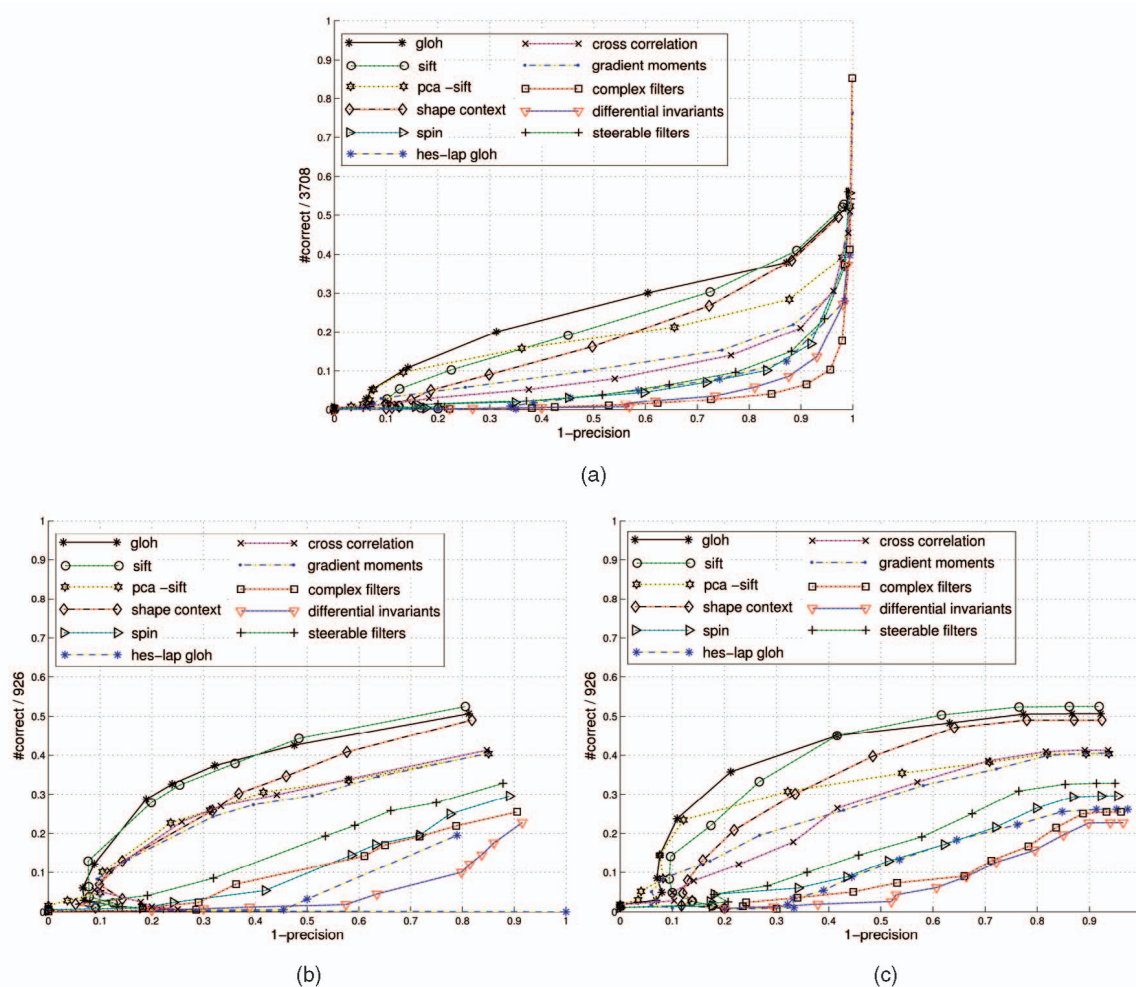
Fig. 4. Comparison of different matching strategies. Descriptors computed on Hessian-Affine regions for images from Fig. 3e. (a) Threshold-based matching. (b) Nearest neighbor distance ratio matching. (c) Nearest neighbor matching. hes-lap gloh is the GLOH descriptor computed for Hessian-Laplace regions (cf., Section 4.1.4).
